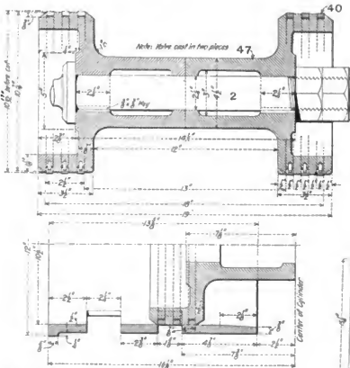
Figs. 2140-2142. Solid Piston Valve for Ten-Wheel (4-6-2) Locomotive with 20 in. x 28 in. Cylinders. Atchafson, Topeka & Santa Fe.
